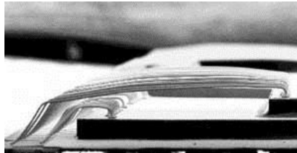
Figure 5. Forward ball bonding loops in stacked die applications.
