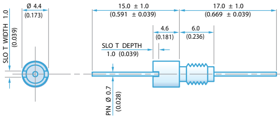
M3.5 x 0.5 - 6g Thread 4.4mm Round Head
