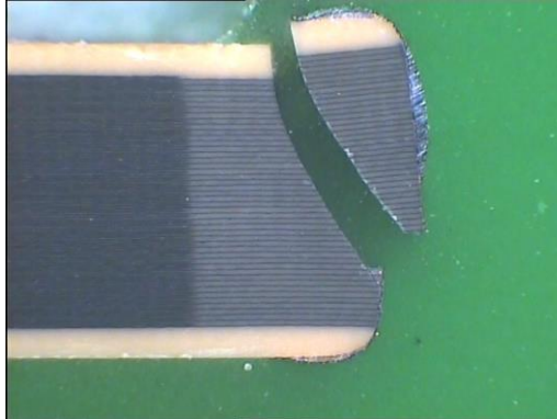
Open Mode Capacitor post bend and 85°C/85%RH test. Capacitance loss approximately 70%.
