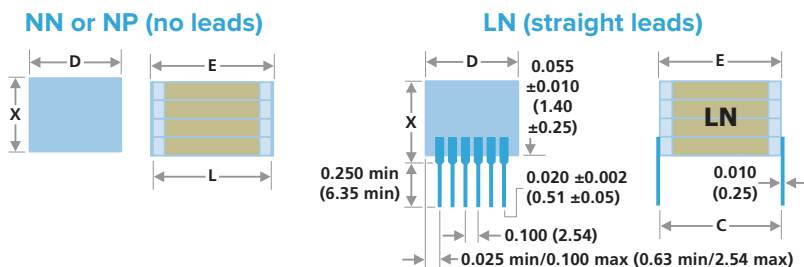
MAXIMUM STACK HEIGHT, X DIMENSION — INCHES/MM
