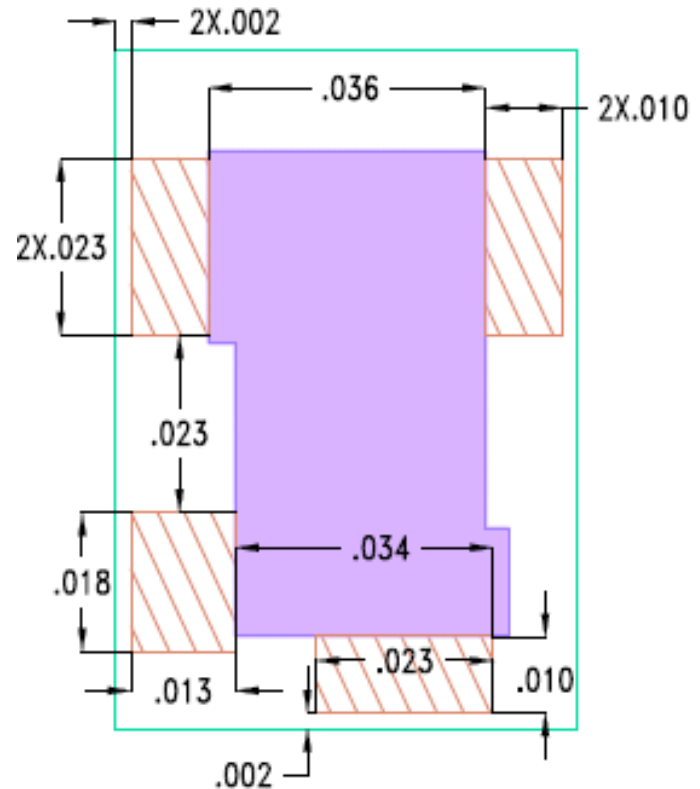
Bottom View
